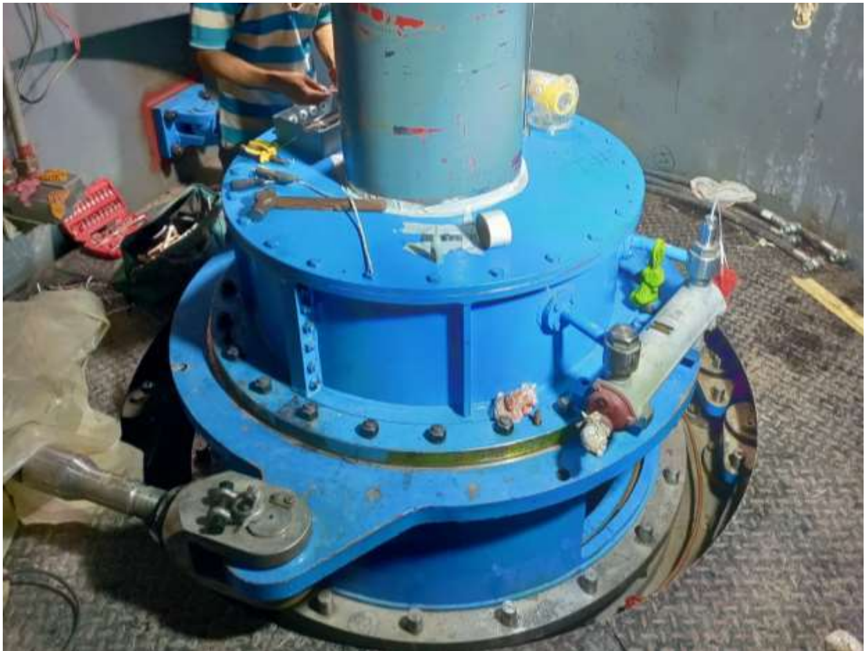
Figure 2-59: Final installation of water guide mechanism along with monitoring sensors
