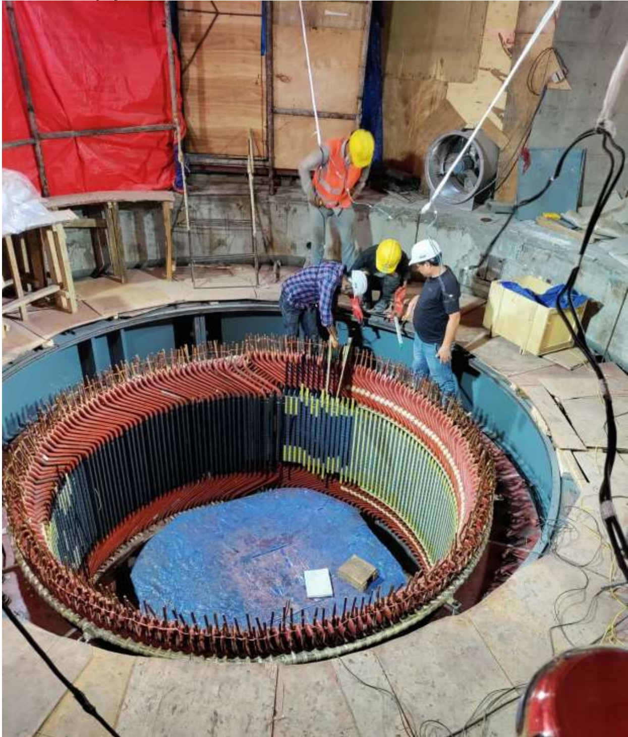
Figure 2-60: High voltage AC test of stator coils
