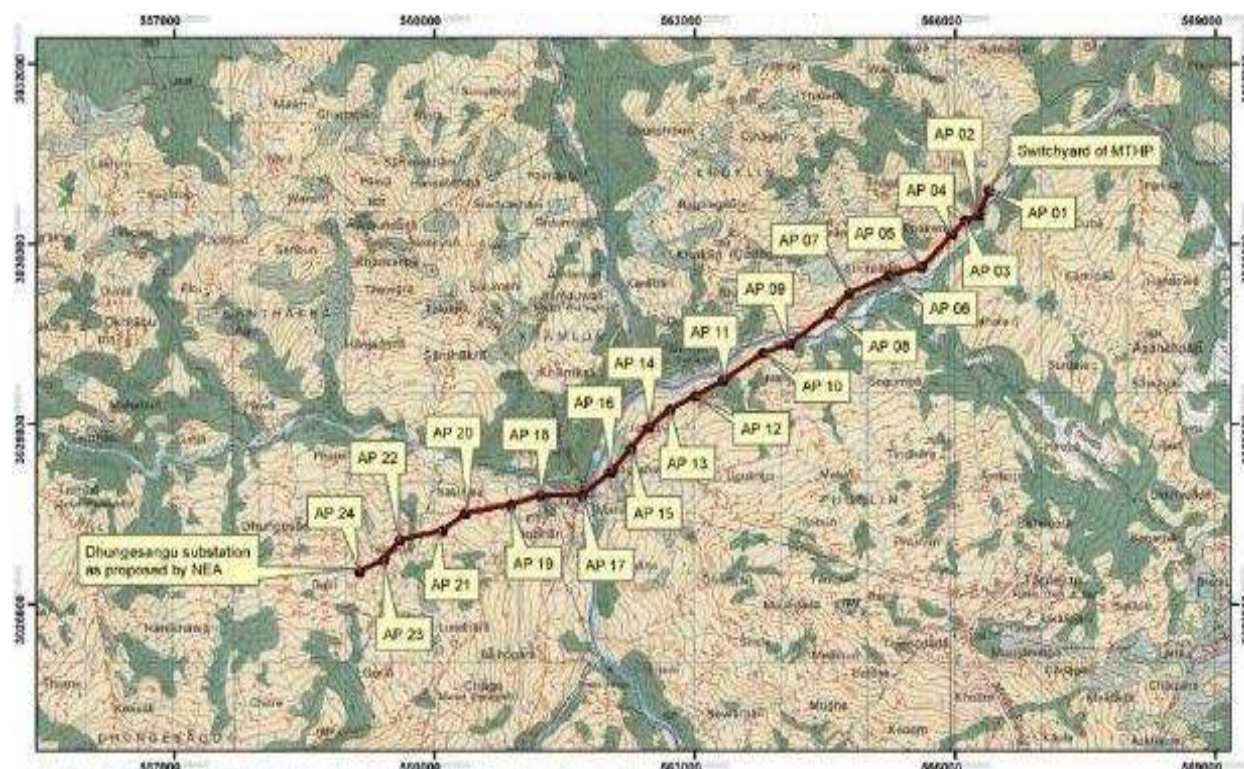
Figure 2-84: Transmission line route map
