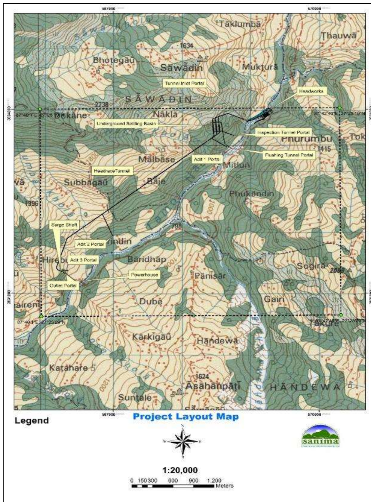
Figure 1-1: General layout of the Project Structures
