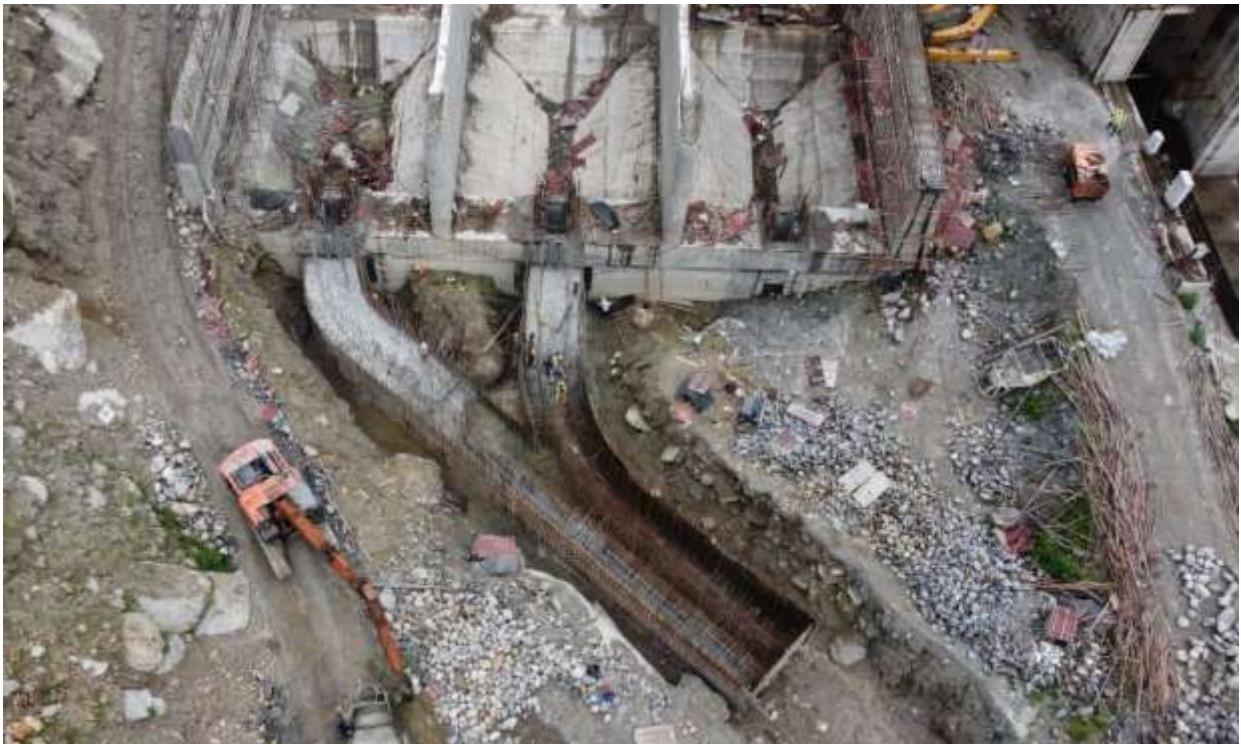
Figure 9: Rebar and concrete works in gravel flushing culvert
