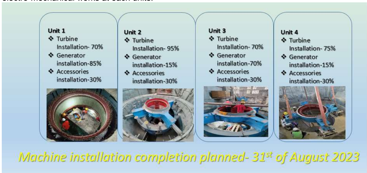
Figure 2-40: Summary of Machine installation
