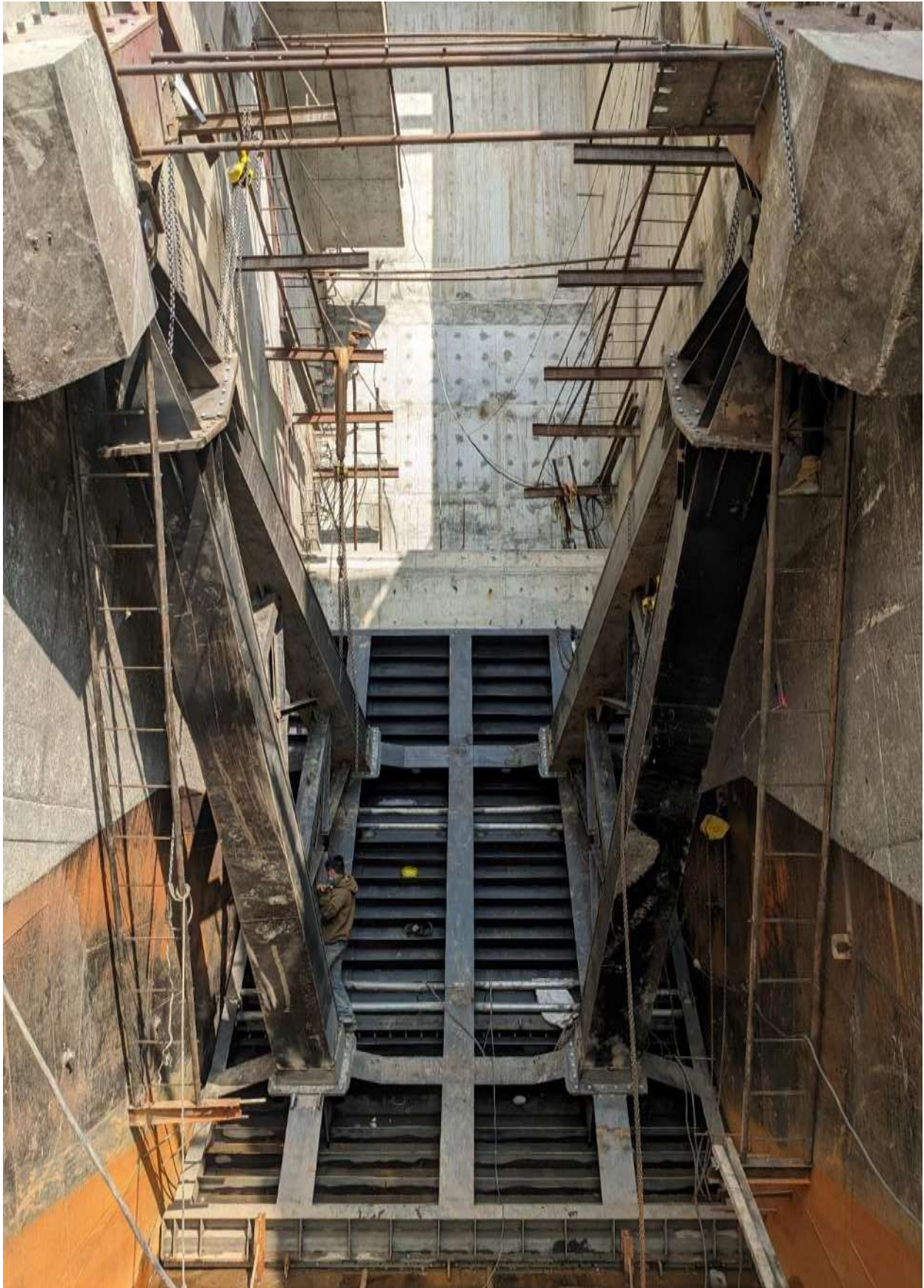
Figure 2-32: Erection of radial gate (installation of seal is remaining)
