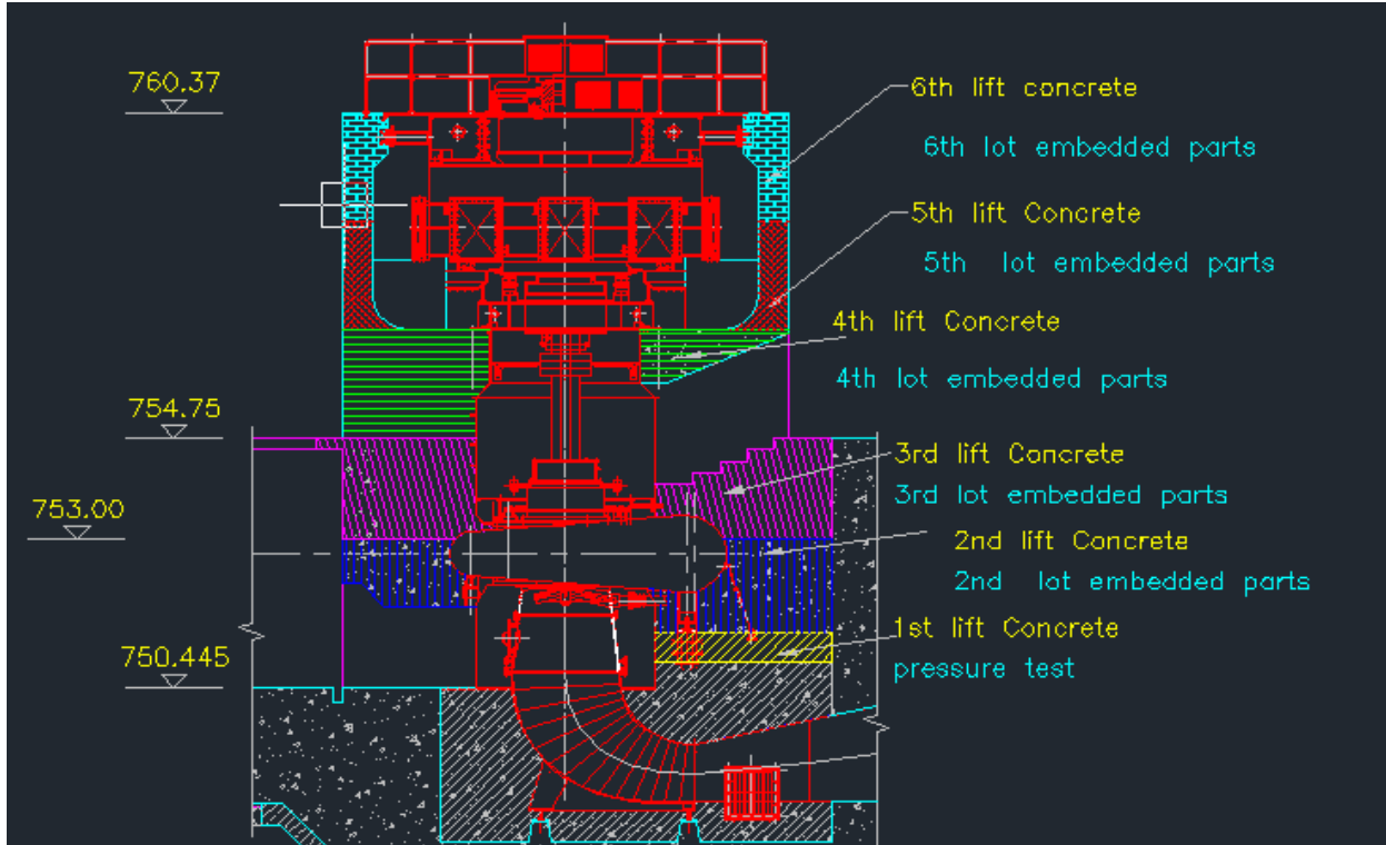
Figure 2-39: Picture showing installation interface between Civil and EM Works
