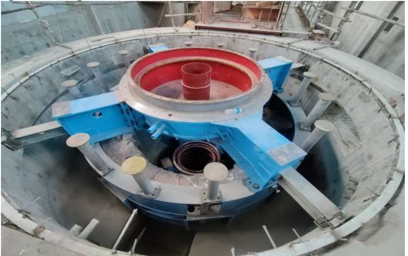
Figure 61: Preassembly of upper bracket and floor components
