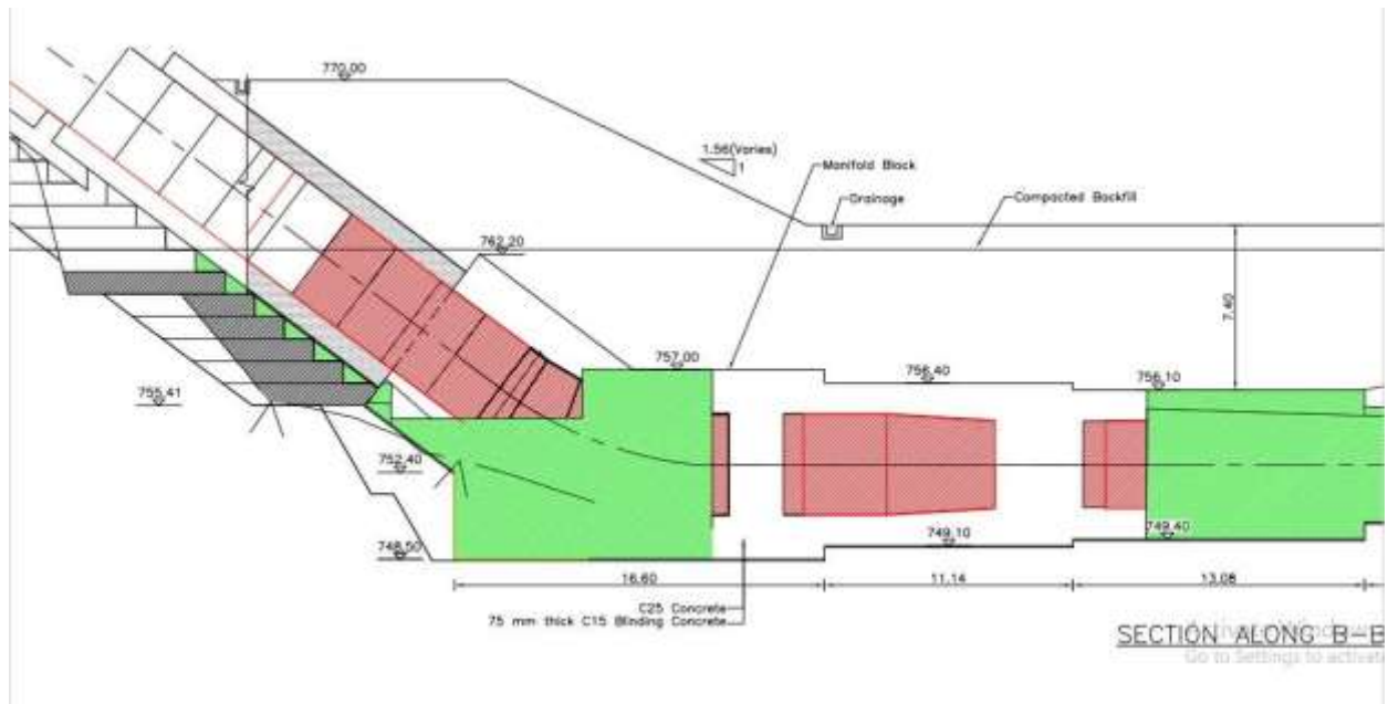
Figure 2-31: Manifold concrete progress
