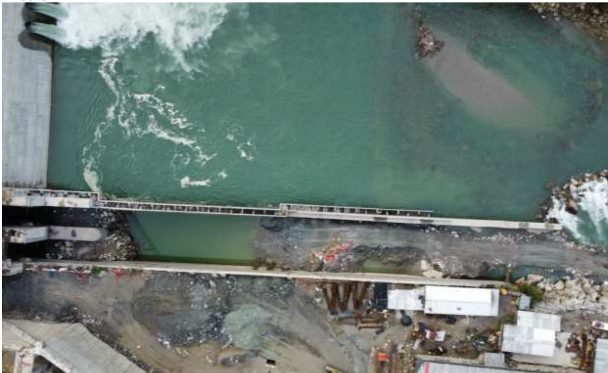
Figure 2-9: A view of undersluice downstream (bottom), fish ladder (middle) and stilling basin (top)
