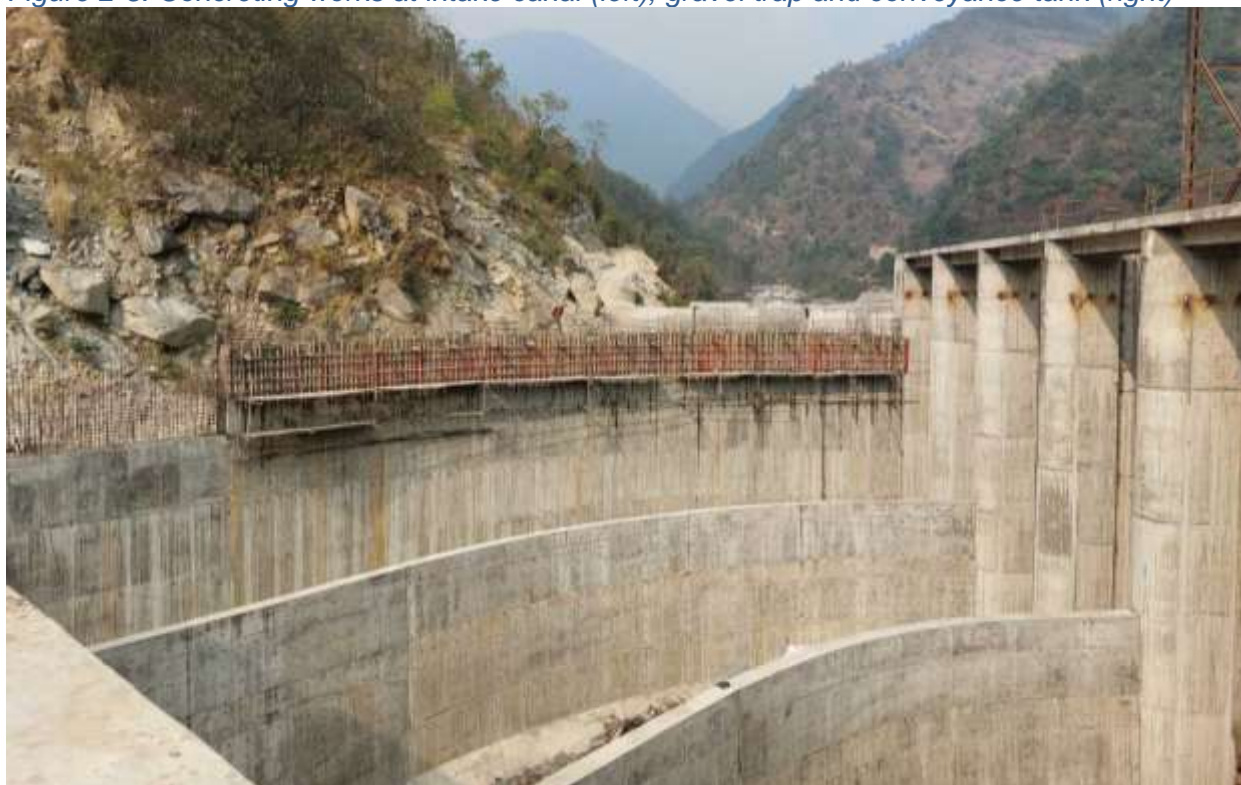
Figure 2-6: Rebar layout at the hillside wall of intake
