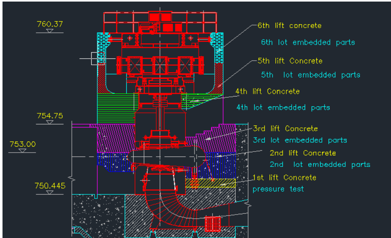
Figure 2-54: Picture showing installation interface between Civil and EM Works
