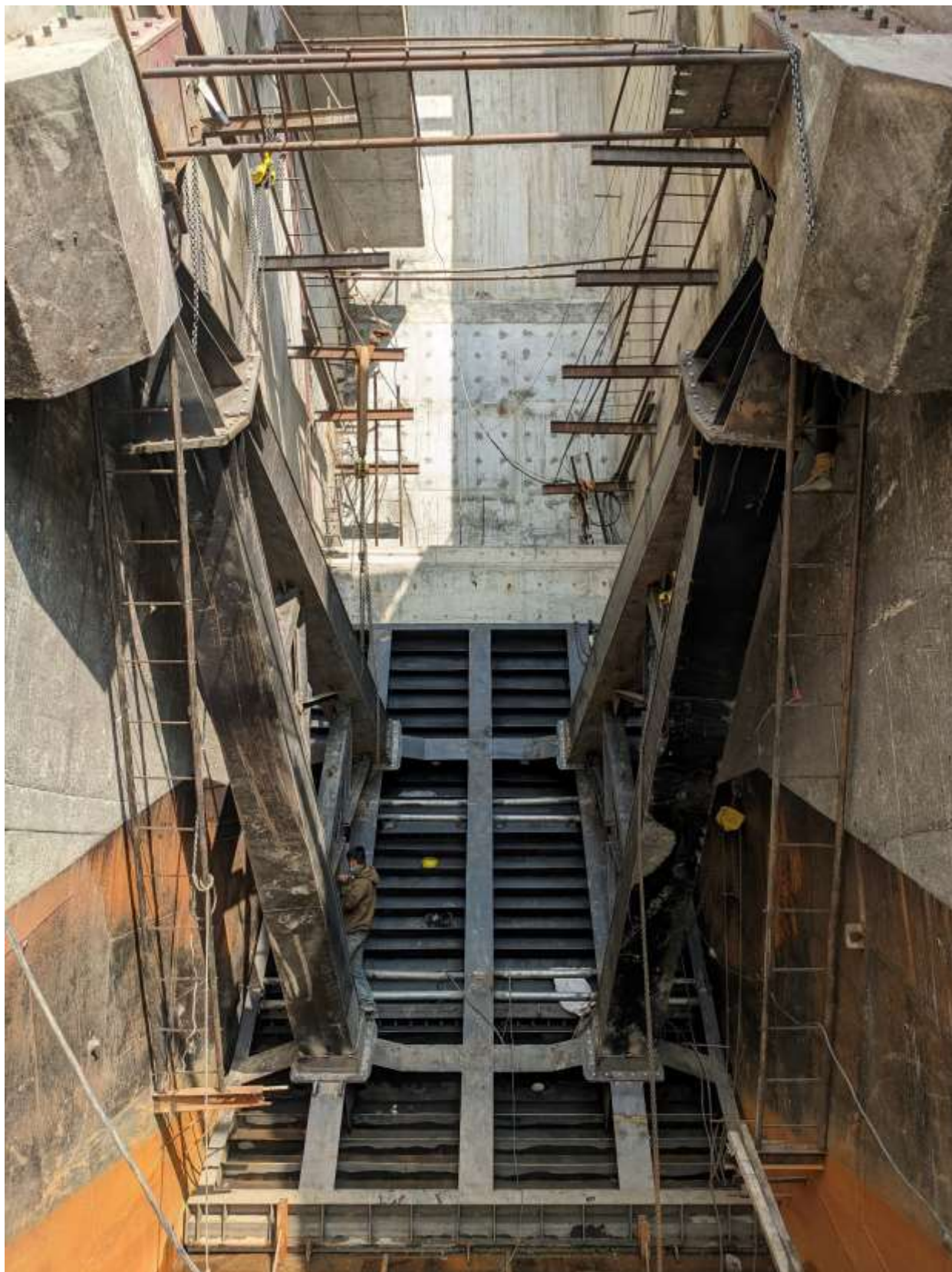
Figure 2-44: Erection of radial gate (installation of seal is remaining)
